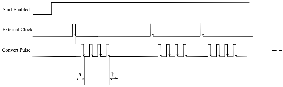
Figure 6.4 Grouping sampling under the not fixed frequency external clock mode
